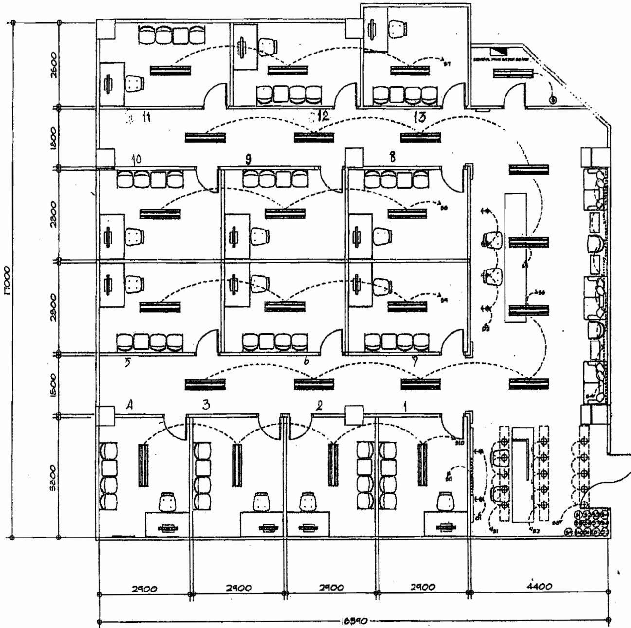
ELECTRICAL LAY'OUT PLAN SCALE 1:100 5th FLOOR
